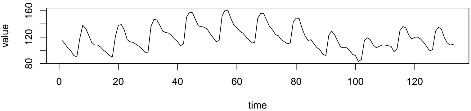
Working Time Series ( \lambda=1, d=0, D=0 )
