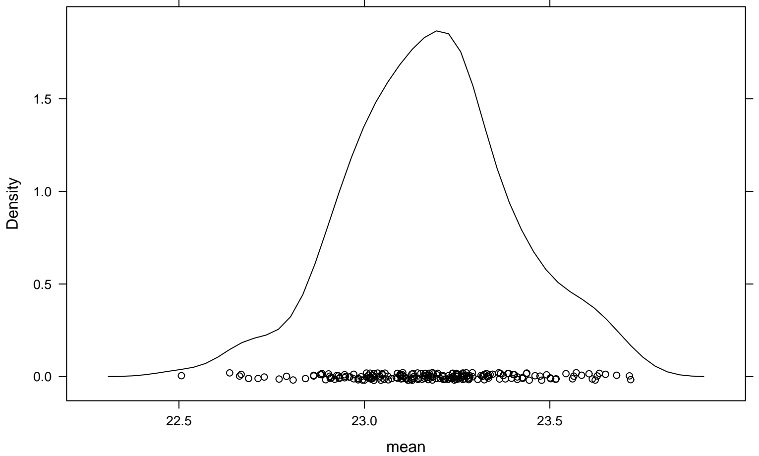
Density Plot
