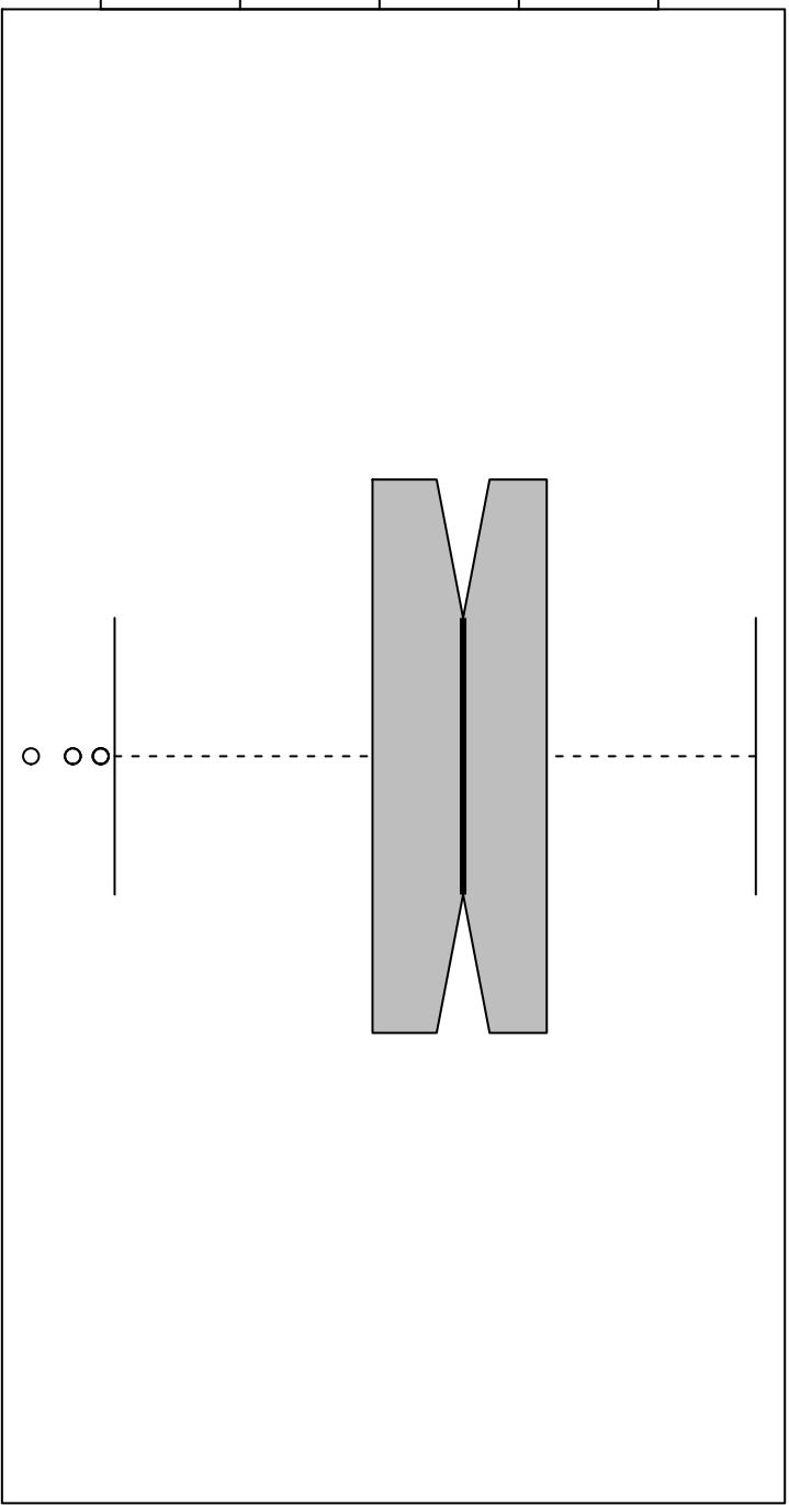
Notched Boxplots
