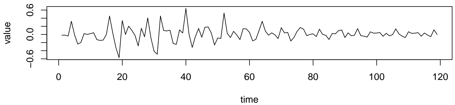
Working Time Series ( \lambda=0 , d=1 , D=0 )
