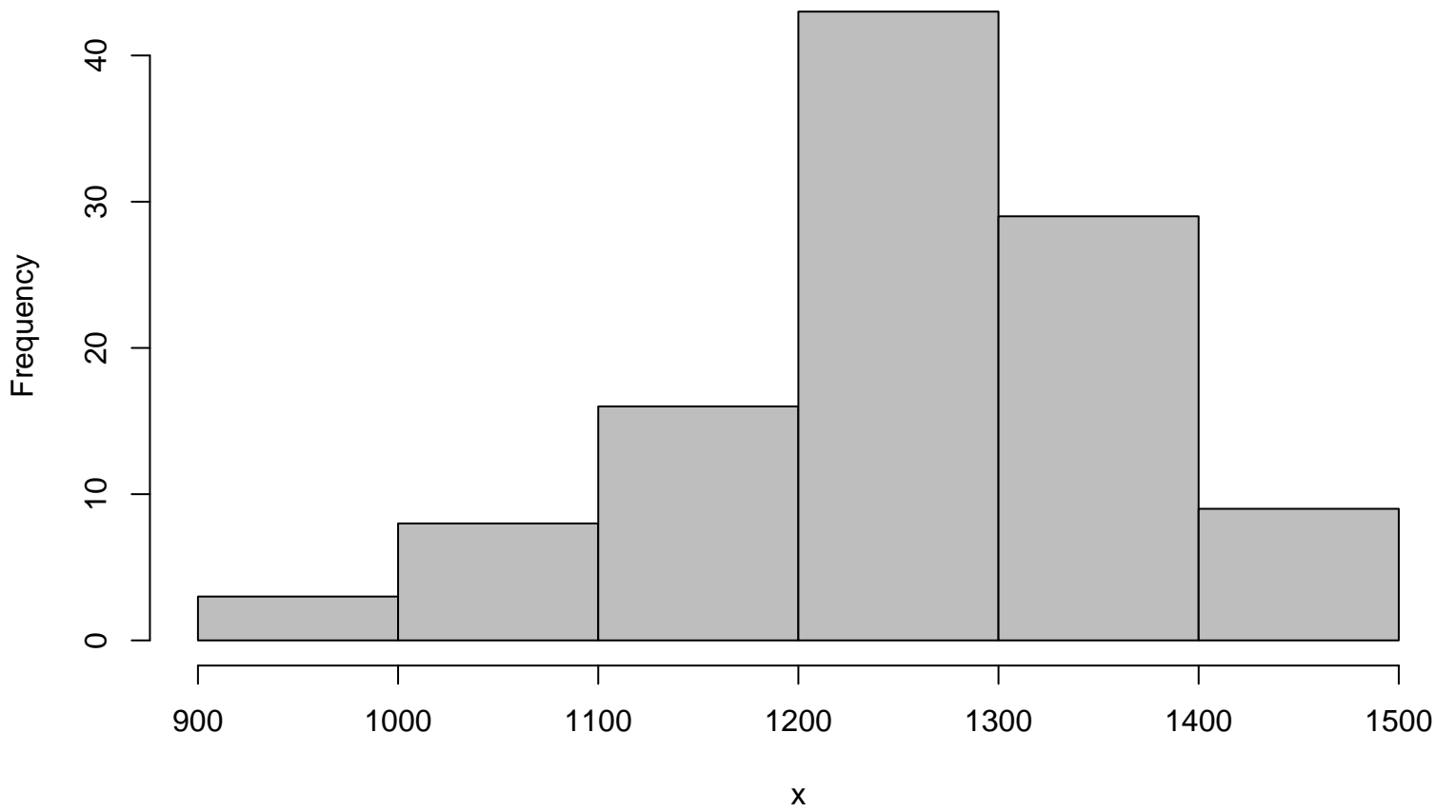
Histogram
