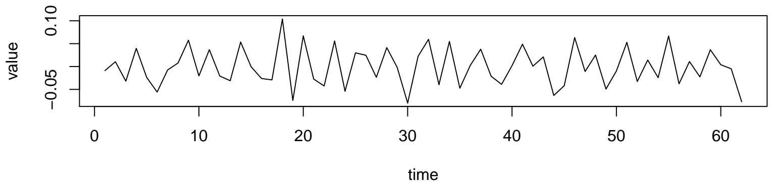
Working Time Series ( \lambda=0, d=1, D=1 )
