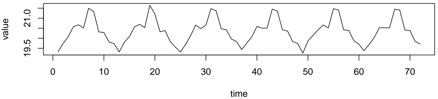
Working Time Series (base=2, d=0, D=0)
