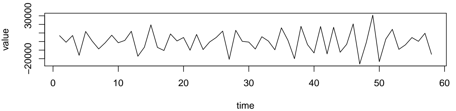
Working Time Series ( \lambda=1 , d=2 , D=2 )
