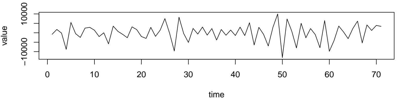
Working Time Series (lambda=1, d=1, D=1)
