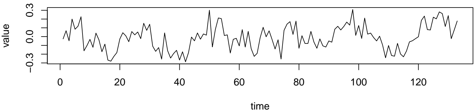
Working Time Series ( \lambda=0 , d=0 , D=1 )
