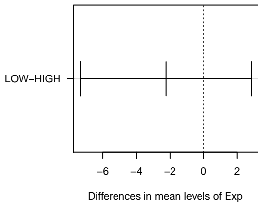
95% family-wise confidence level
