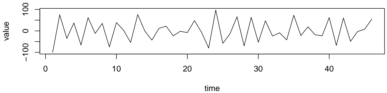
Working Time Series ( \lambda=1, d=2, D=2 )
