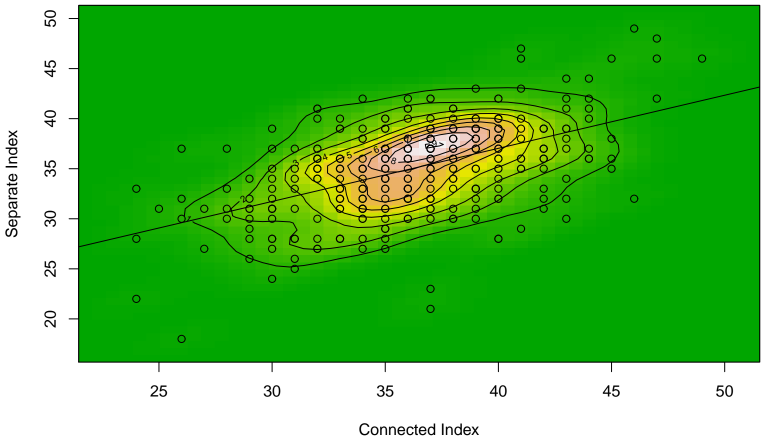
Bivariate Kernel Density – Ubiq. Study
