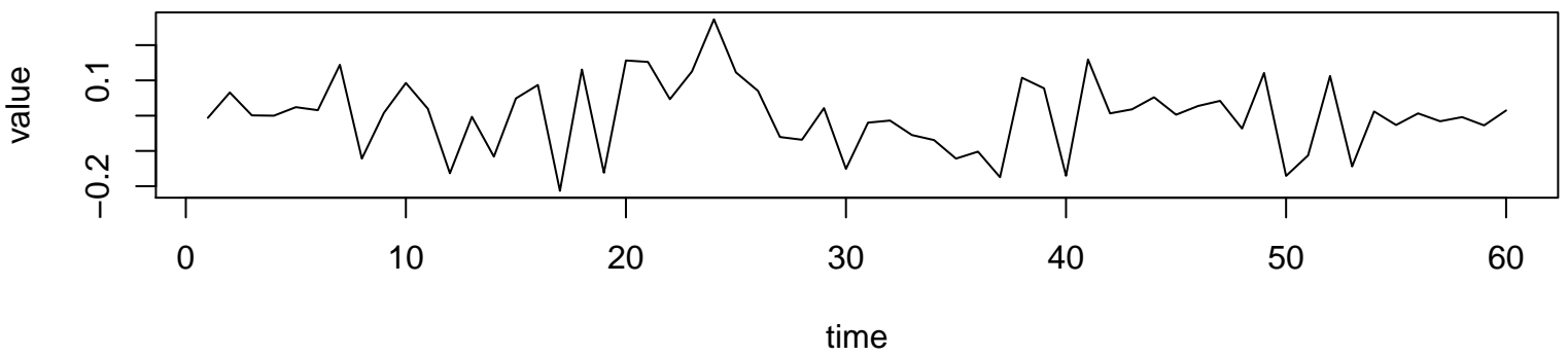
Working Time Series (base=2, d=0, D=1)
