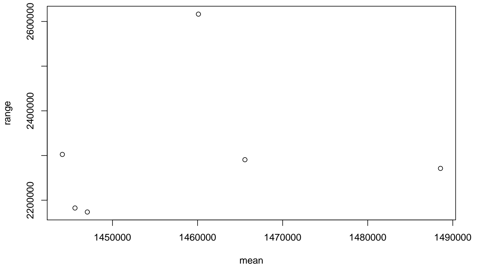
Range-Mean Plot
