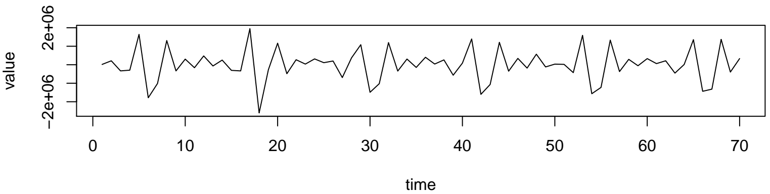
Working Time Series ( \lambda=1 , d=2 , D=0 )
