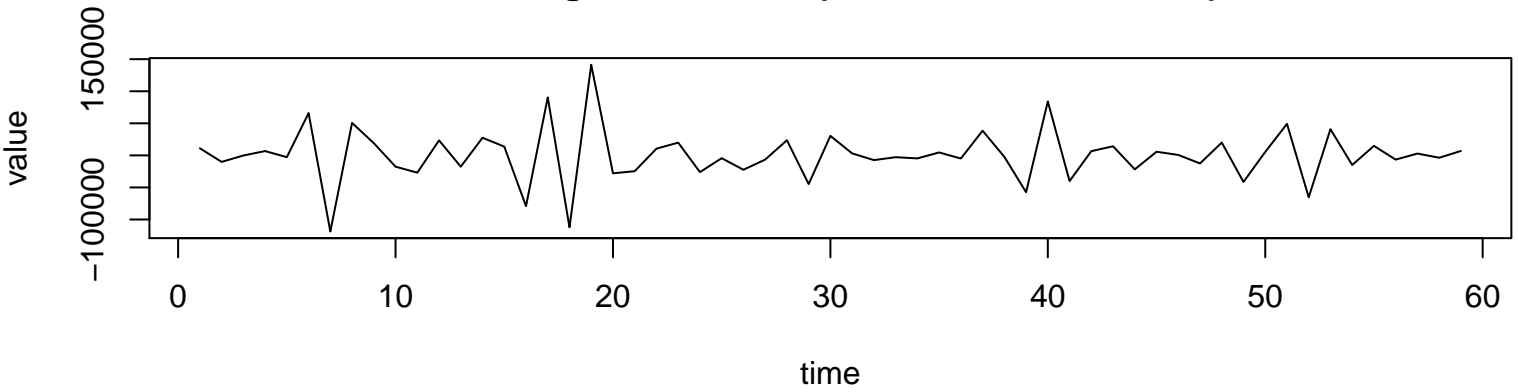
Working Time Series ( \lambda=0.9 , d=1 , D=1 )
