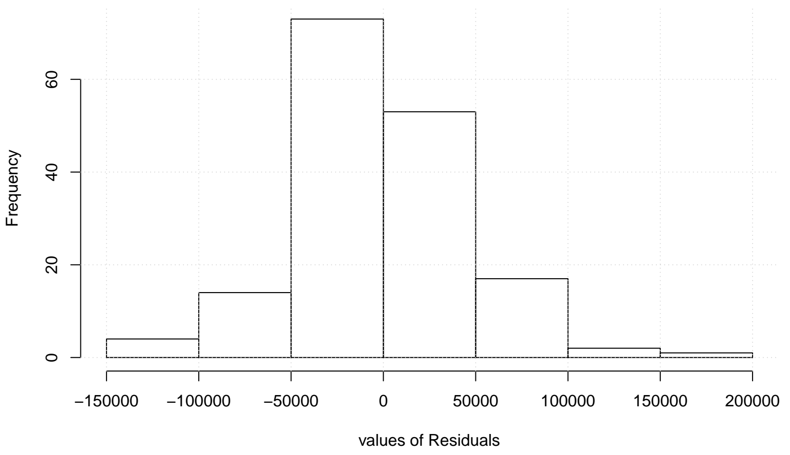
Residual Histogram
