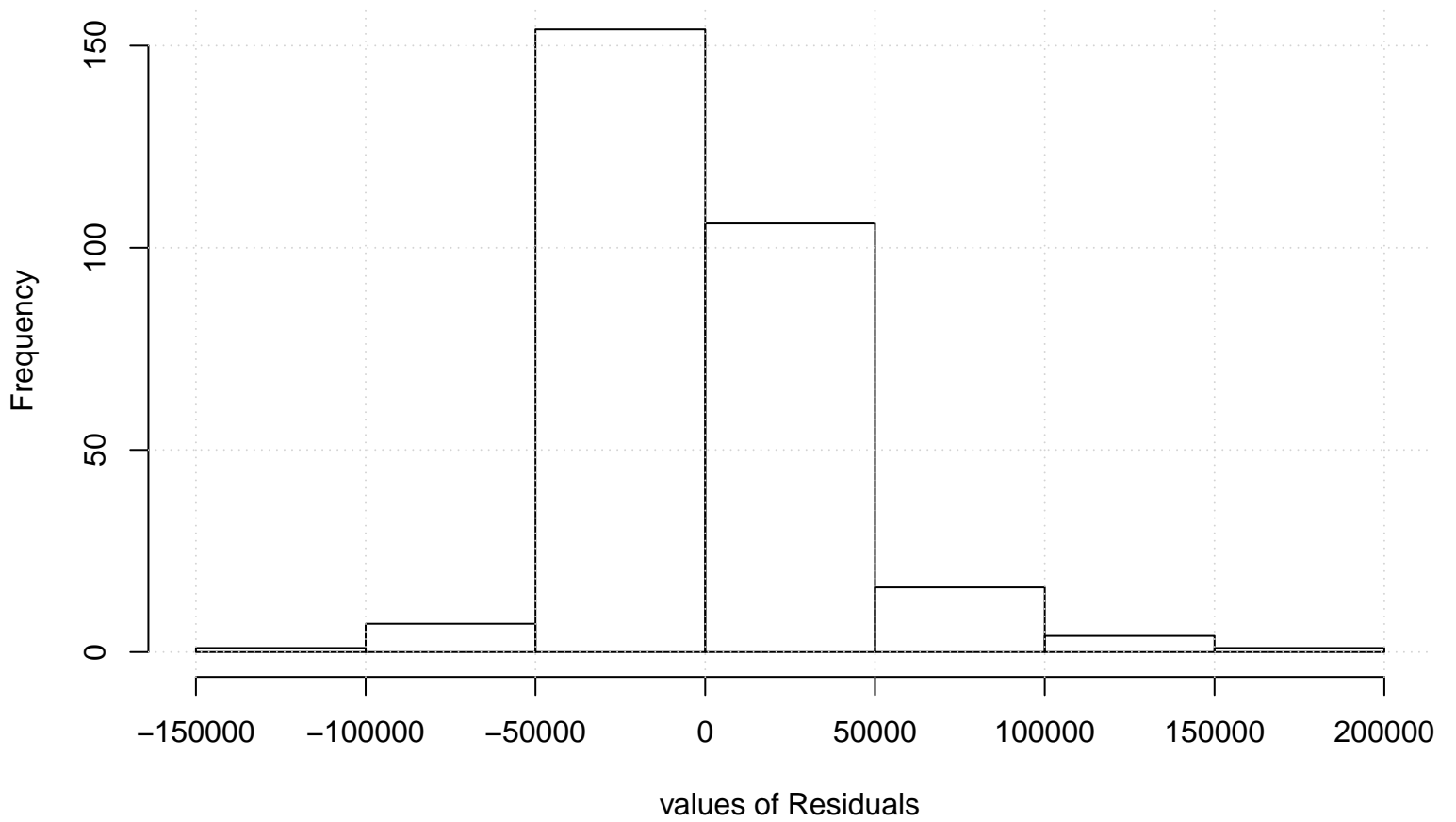
Residual Histogram
