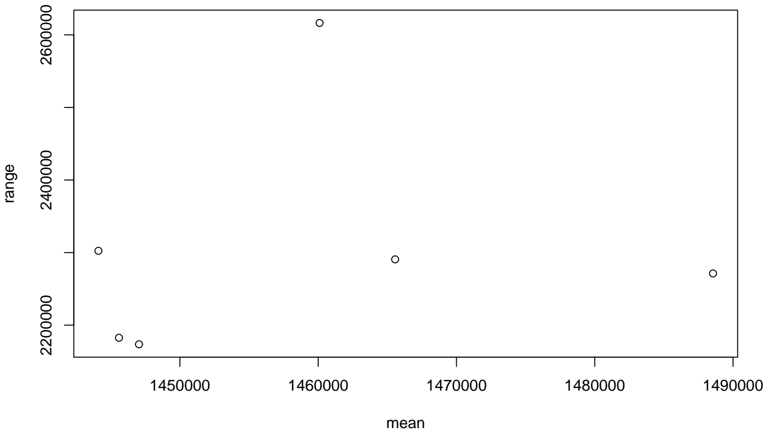
Range–Mean Plot
