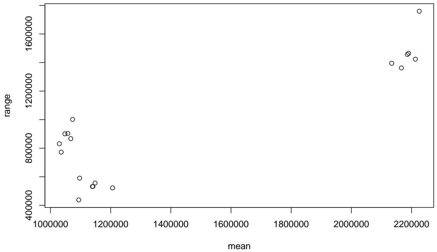
Range-Mean Plot
