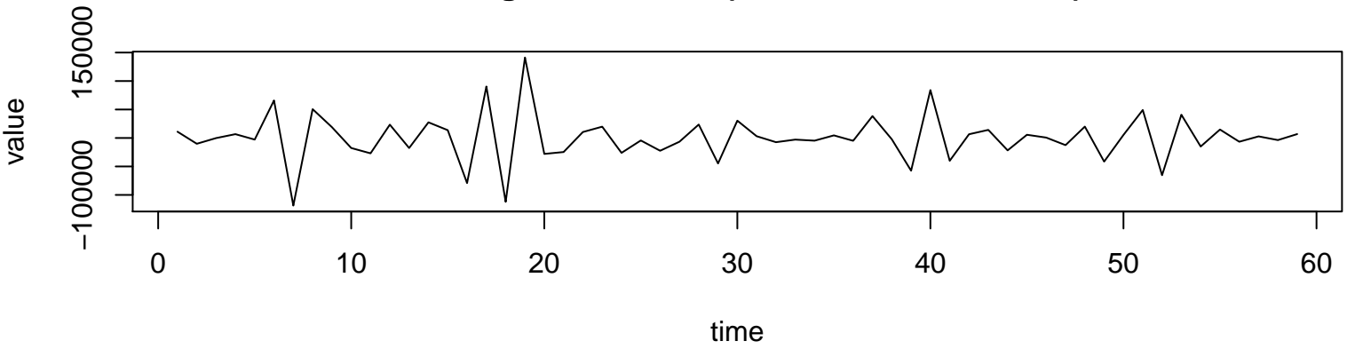
Working Time Series (lambda=0.9, d=1, D=1)
