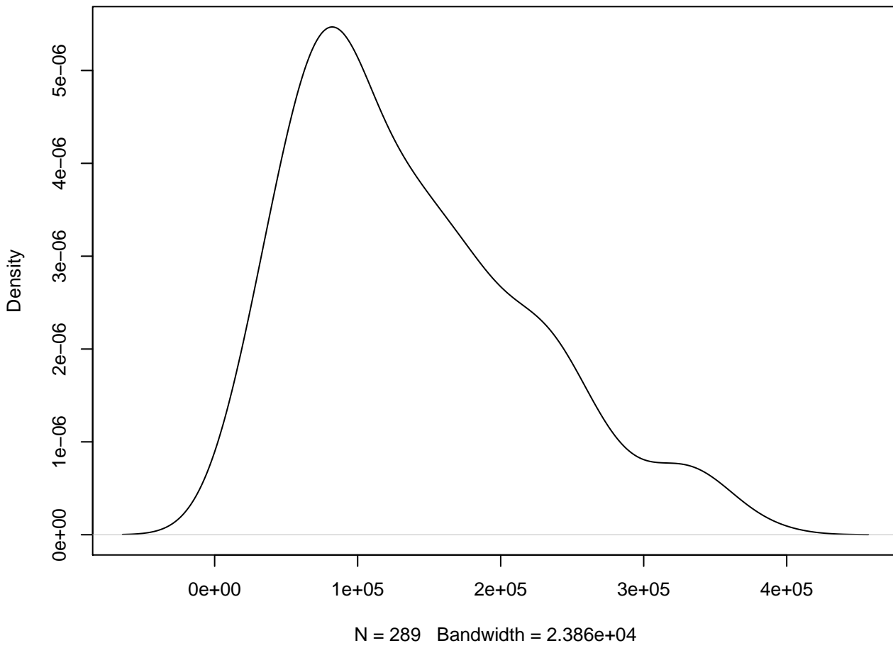
Kernel Density Plot of Actuals
