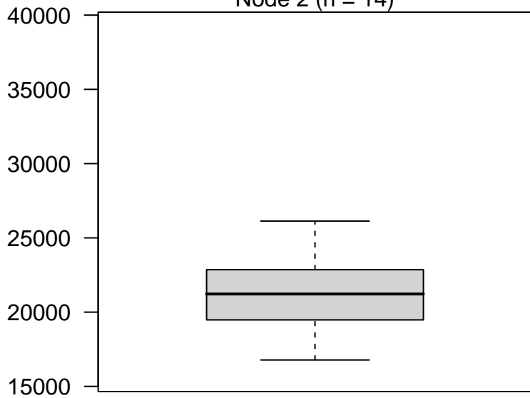
Node 2 (n = 14)
