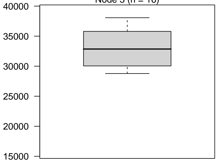
Node 3 (n = 16)
