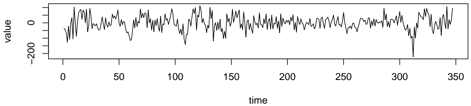
Working Time Series ( \lambda=1 , d=1 , D=2 )
