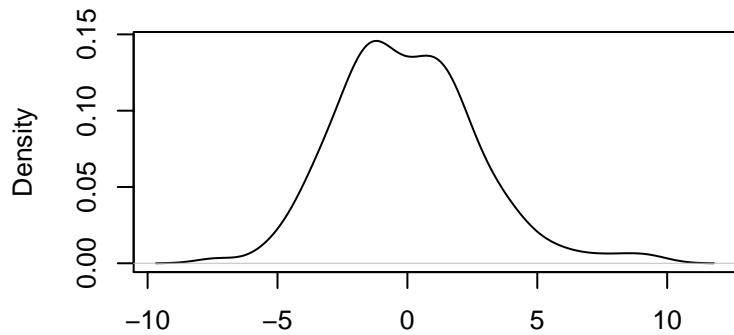
Kernel Density Plot of Residuals
