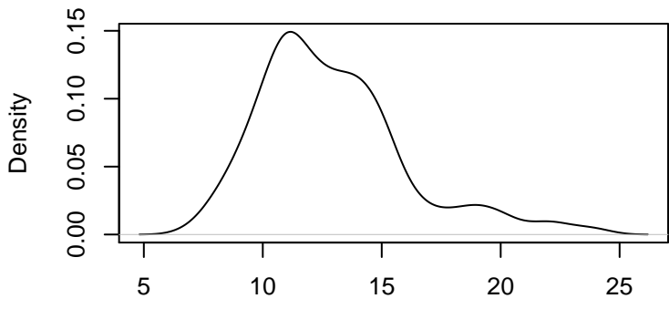
Kernel Density Plot of Actuals
