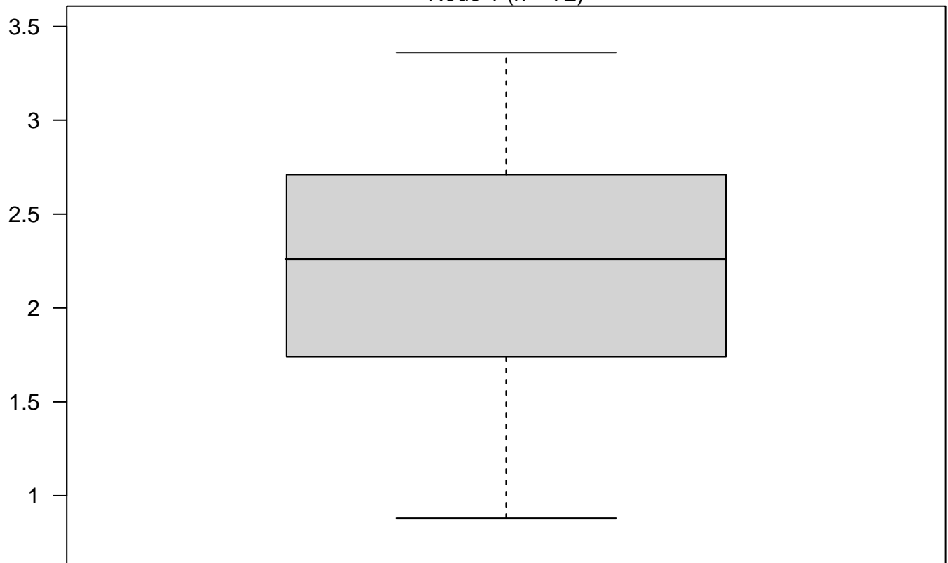
Node 1 (n = 72)
