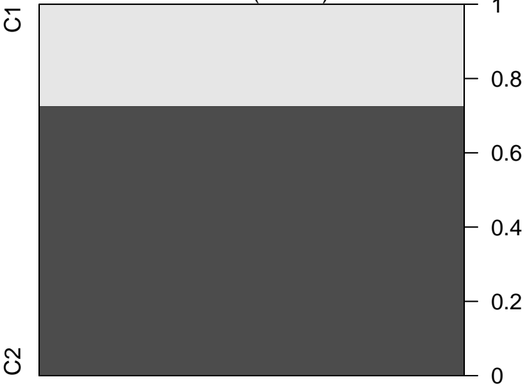
Node 2 (n = 11)
