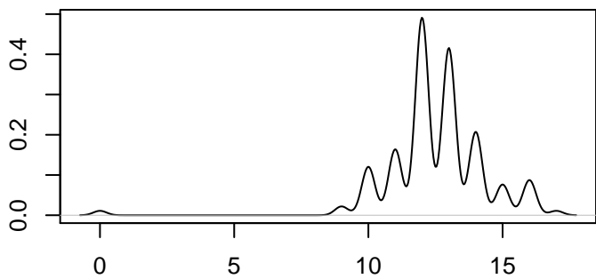
Kernel Density Plot of Actuals
