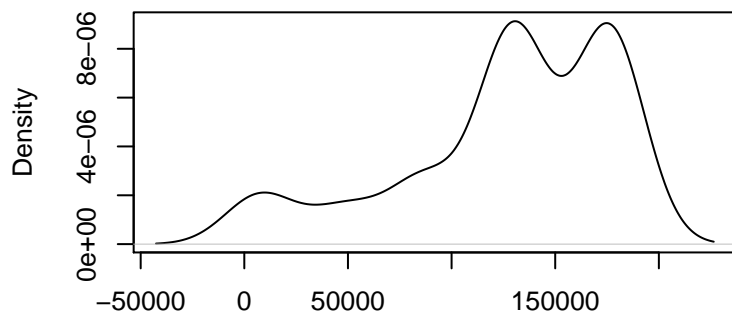
Kernel Density Plot of Predictions
