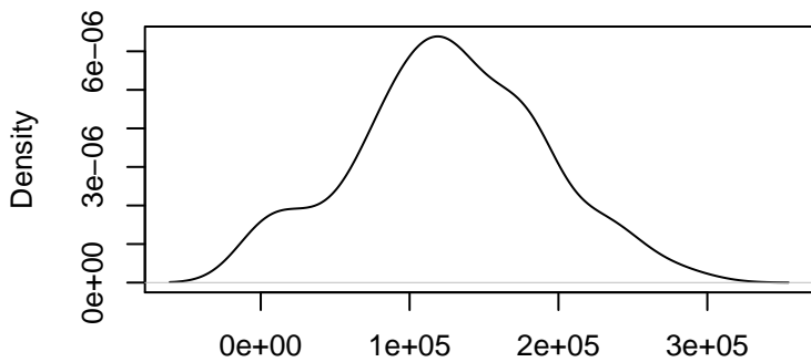
Kernel Density Plot of Actuals
