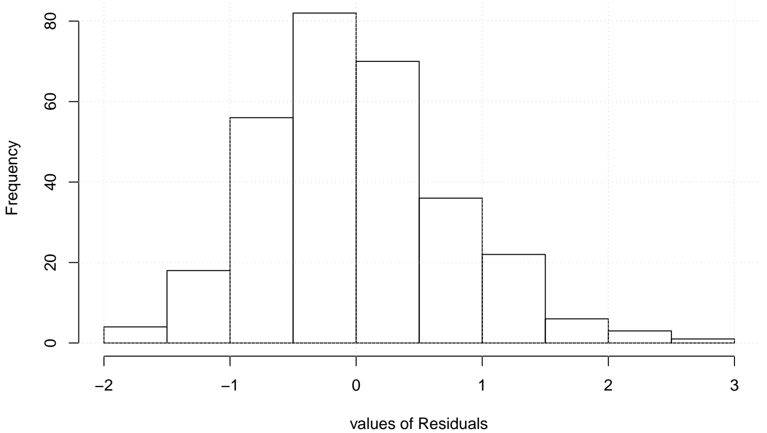
Residual Histogram
