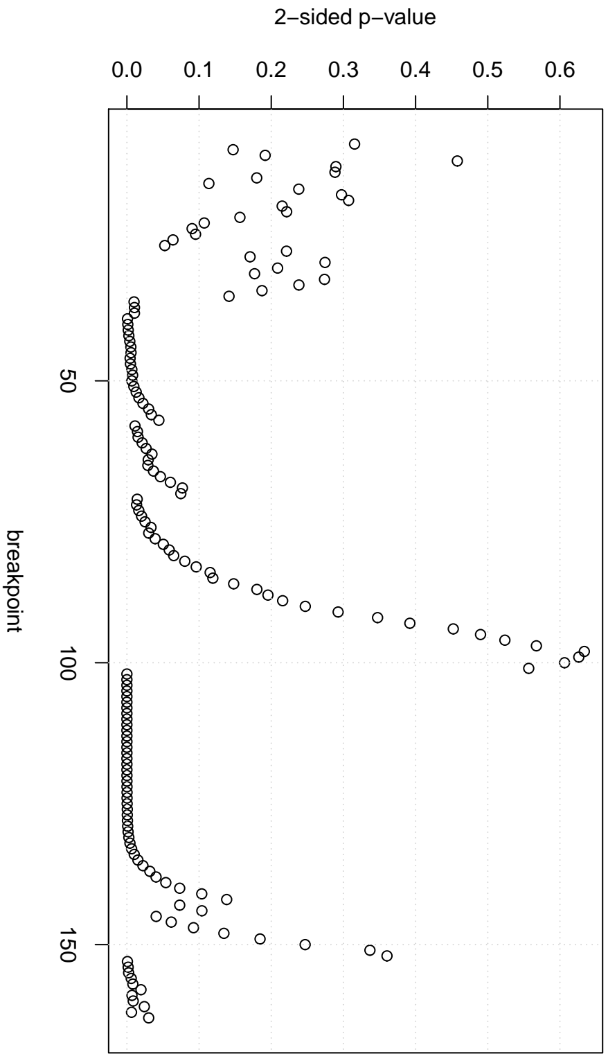
Goldfeld-Quandt test
