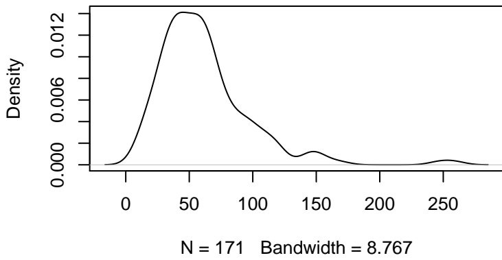
Kernel Density Plot of Actuals
