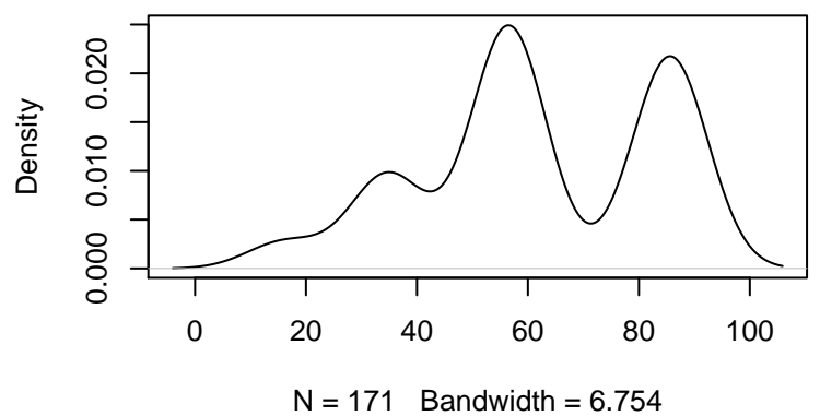
Kernel Density Plot of Predictions
