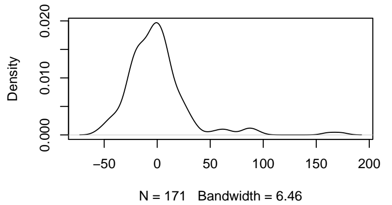
Kernel Density Plot of Residuals
