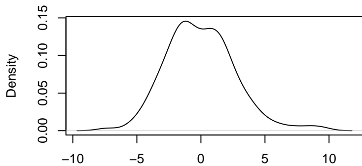
Kernel Density Plot of Residuals
