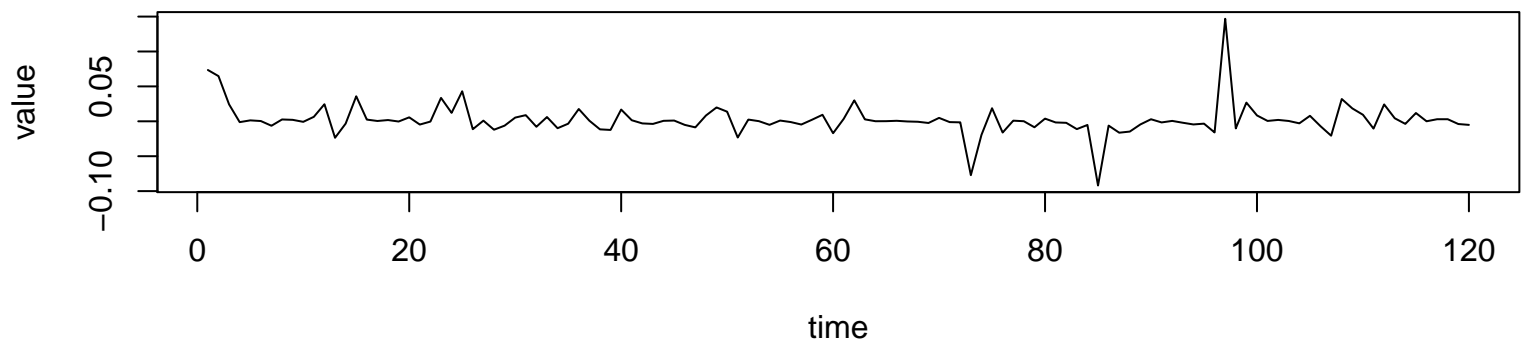
Working Time Series ( \lambda=-2 , d=0 , D=1 )
