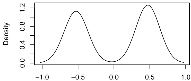
Kernel Density Plot of Residuals
