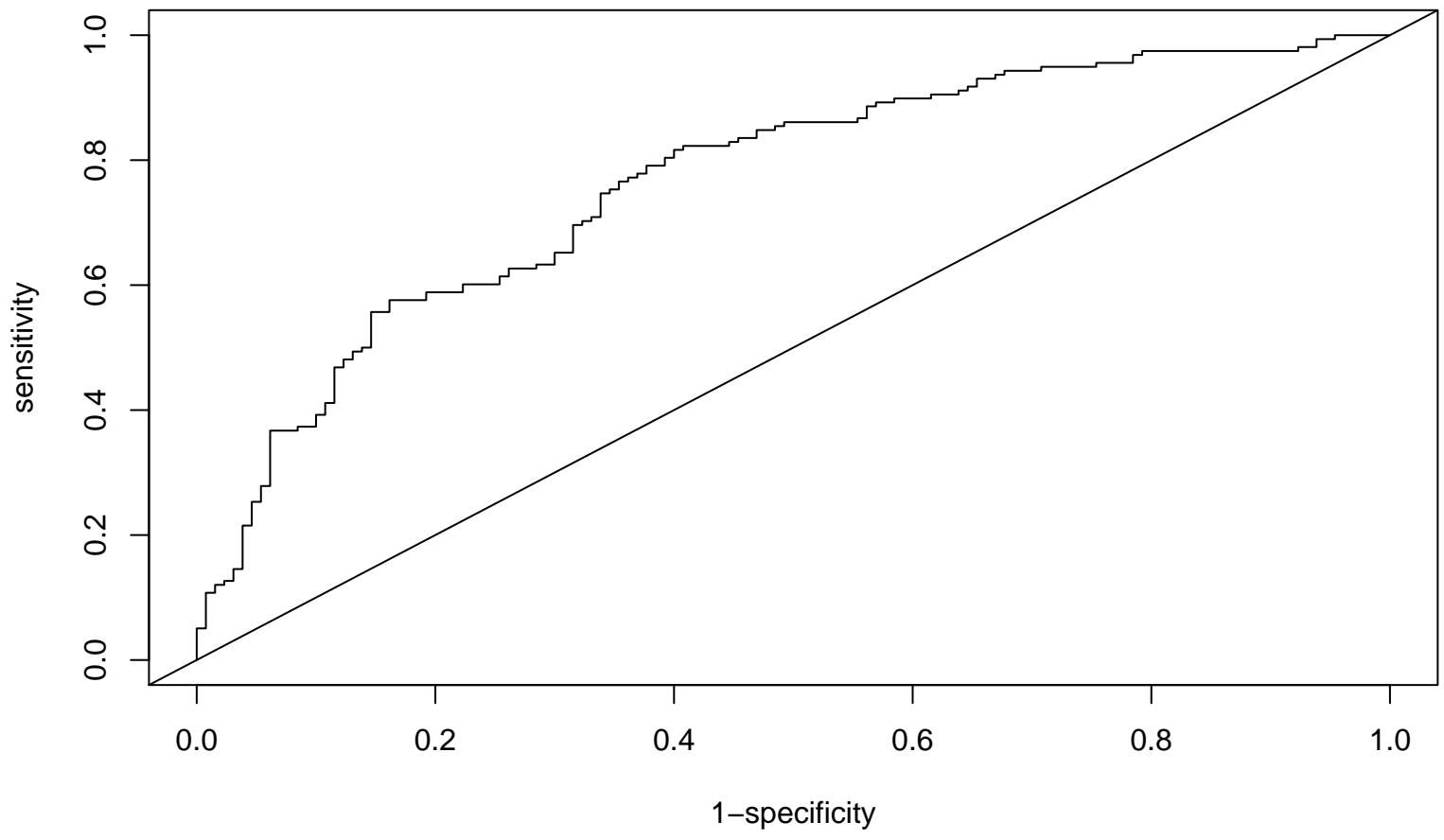
ROC plot
