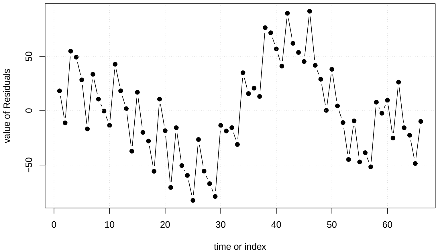
Residuals
