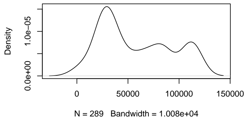
Kernel Density Plot of Predictions
