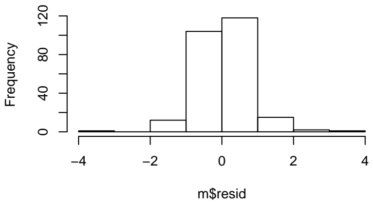
Residual Histogram
