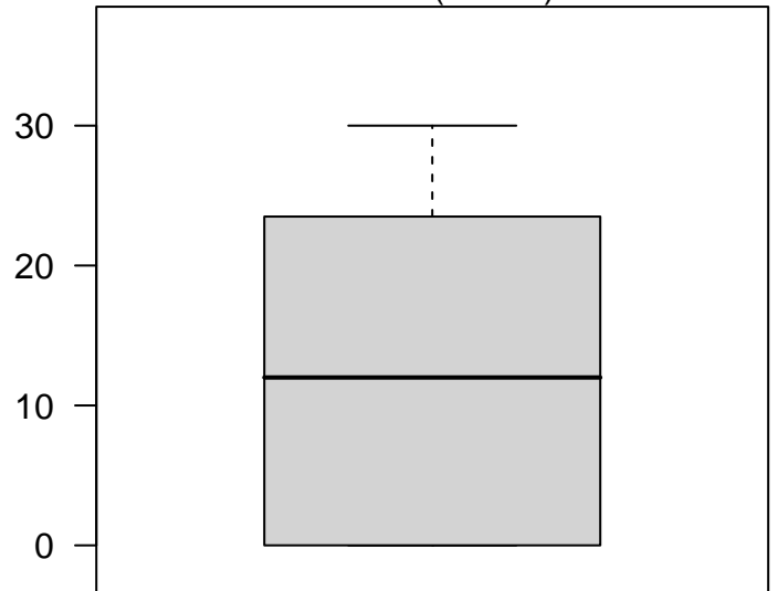
Node 3 (n = 23)
