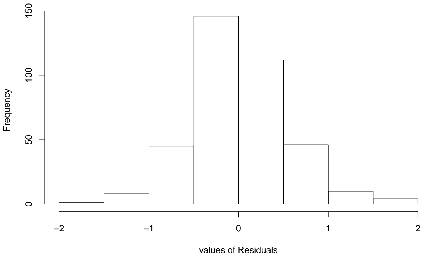
Residual Histogram
