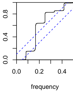
Seasonal
