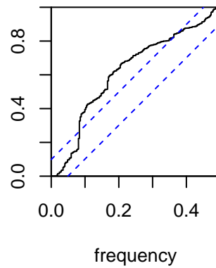
Standardized Residuals
