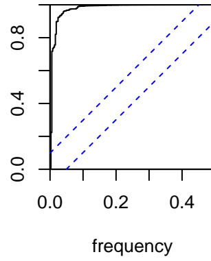
Level
