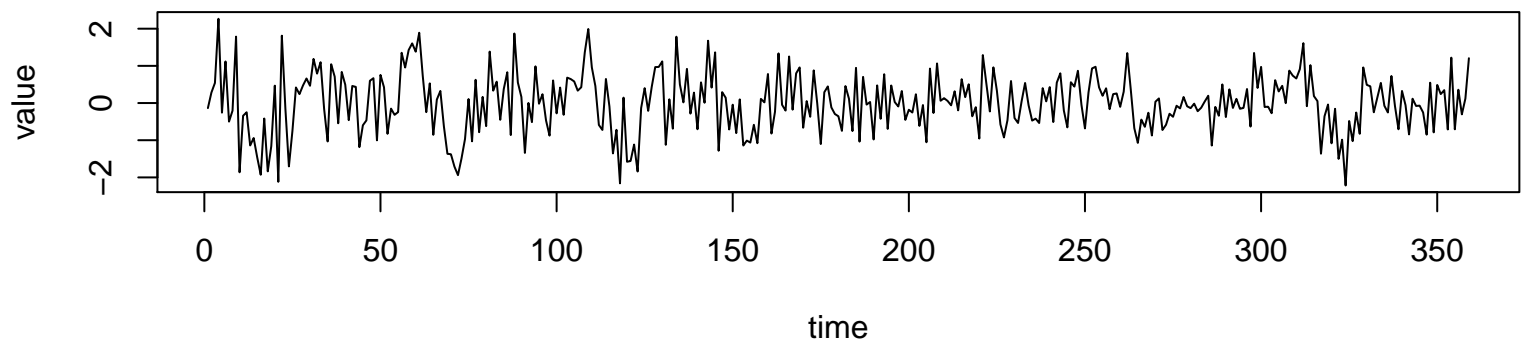
Working Time Series ( \lambda=0.4 , d=1 , D=1 )
