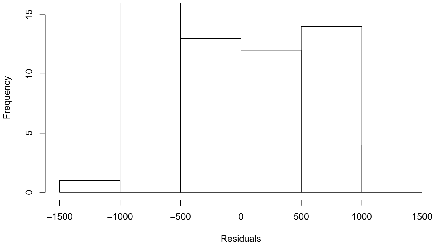
Residual Histogram
