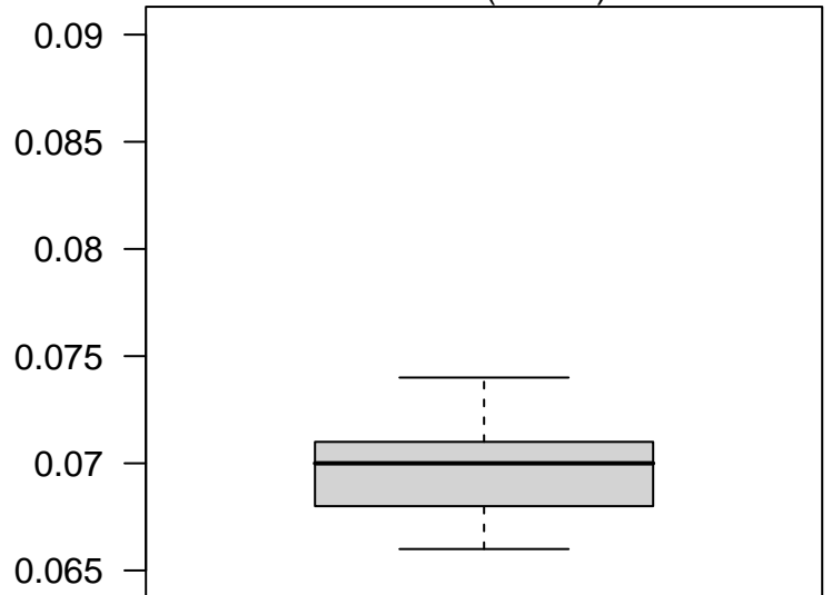
Node 3 (n = 20)
