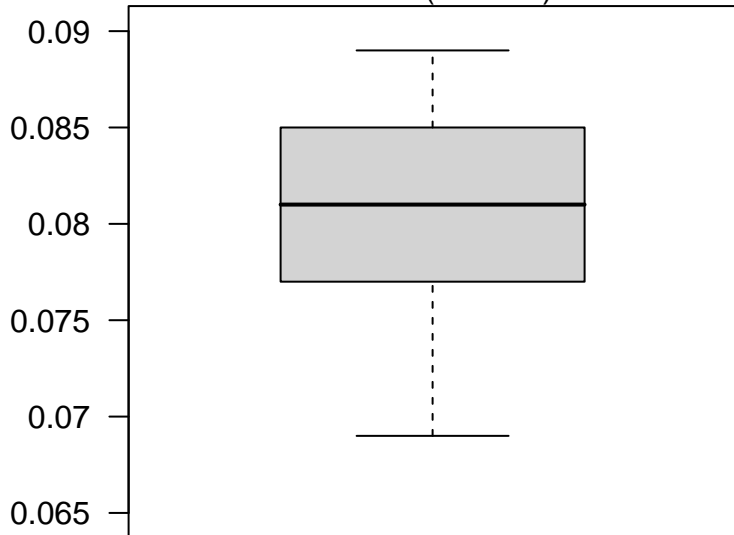
Node 2 (n = 100)
