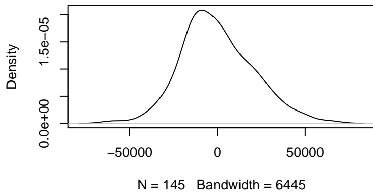
Kernel Density Plot of Residuals
