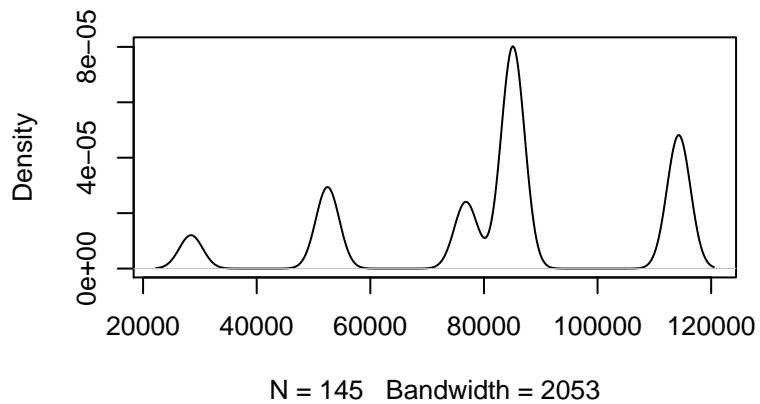
Kernel Density Plot of Predictions
