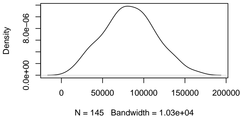
Kernel Density Plot of Actuals
