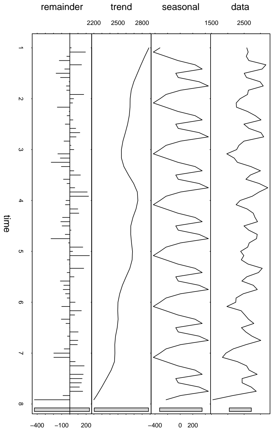
Seasonal Decomposition by Loess
