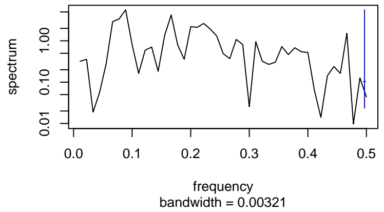
Standardized Residuals
