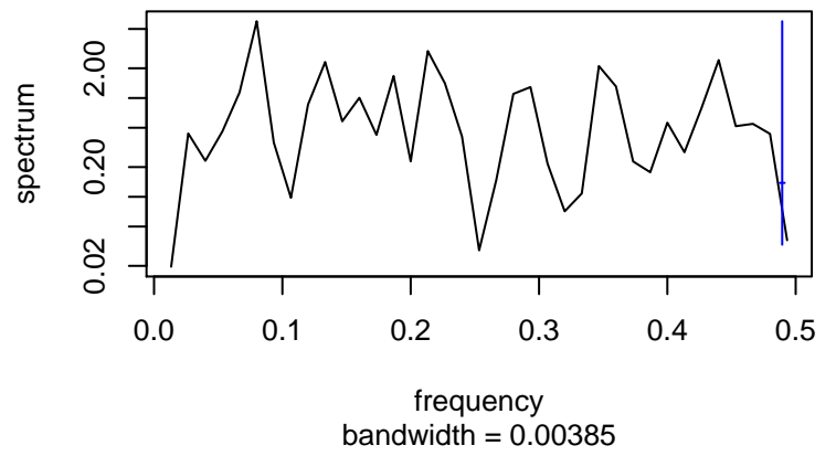
Standardized Residuals
